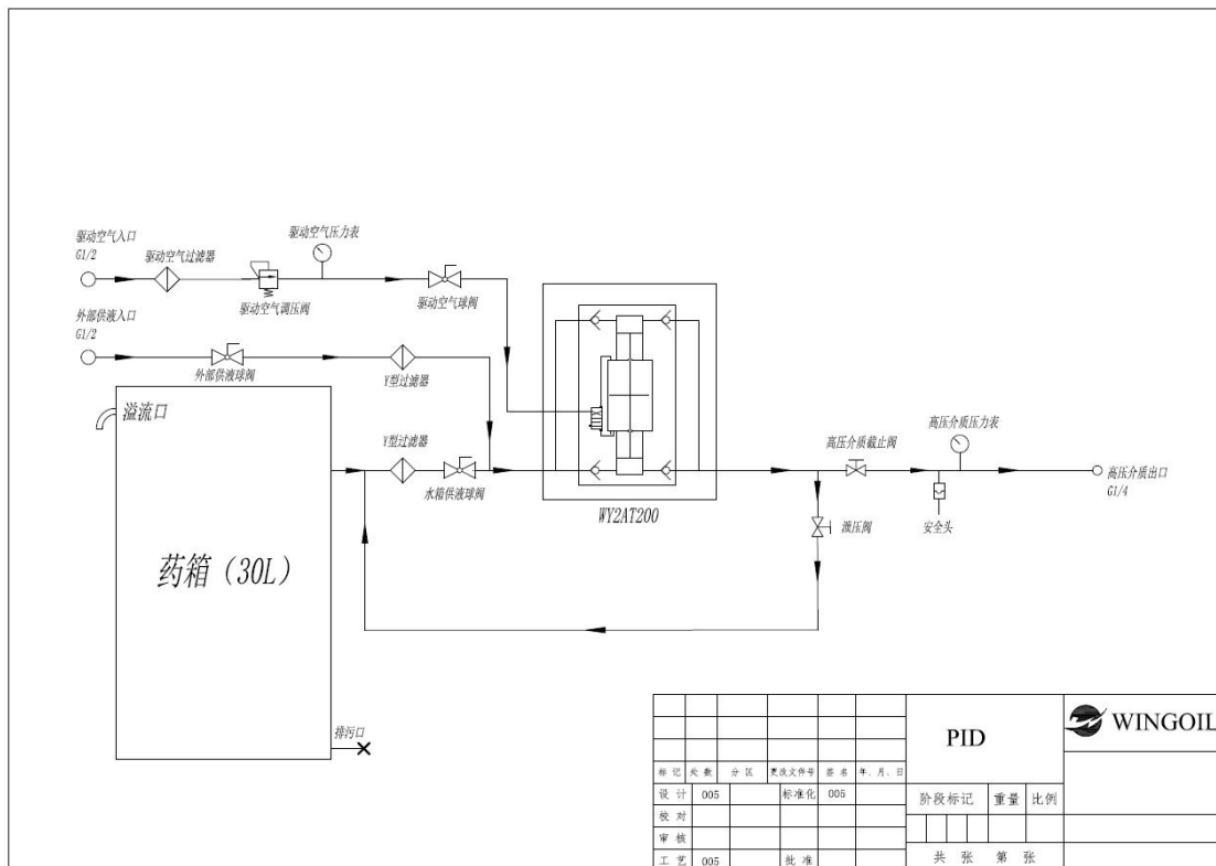
Schematic diagram of fluid part
